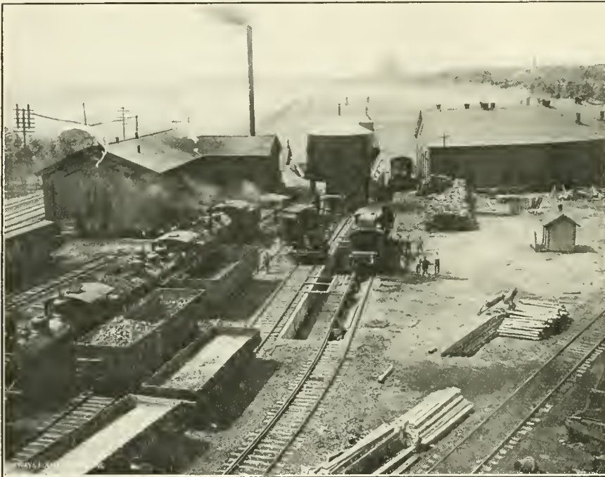
BELLEVUE, O., SHOPS, NICKEL PLATE LINE, WITH CONCRETE CINDER PIT AND CLAM SHELL COALING APPARATUS.
